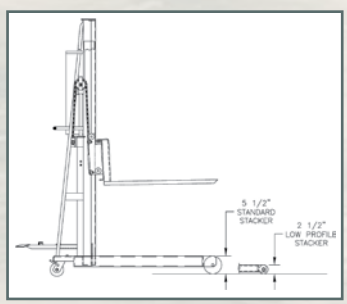
Low Profile Stacker Outtrigger Option, Page 60.
